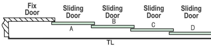
Top View
