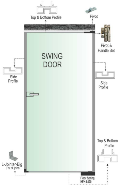
HLX -88 Swing Door
